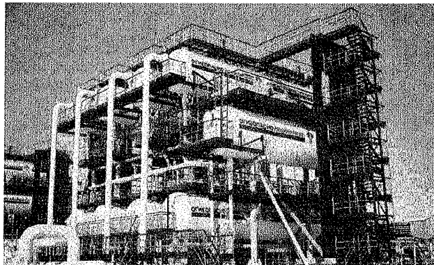
Central processing and pumping facility at the Yuganskneftegaz field, onshore Russia.
