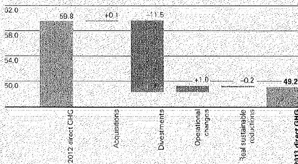
Greenhouse gas emissions (Mta CO 2 equivalent)
