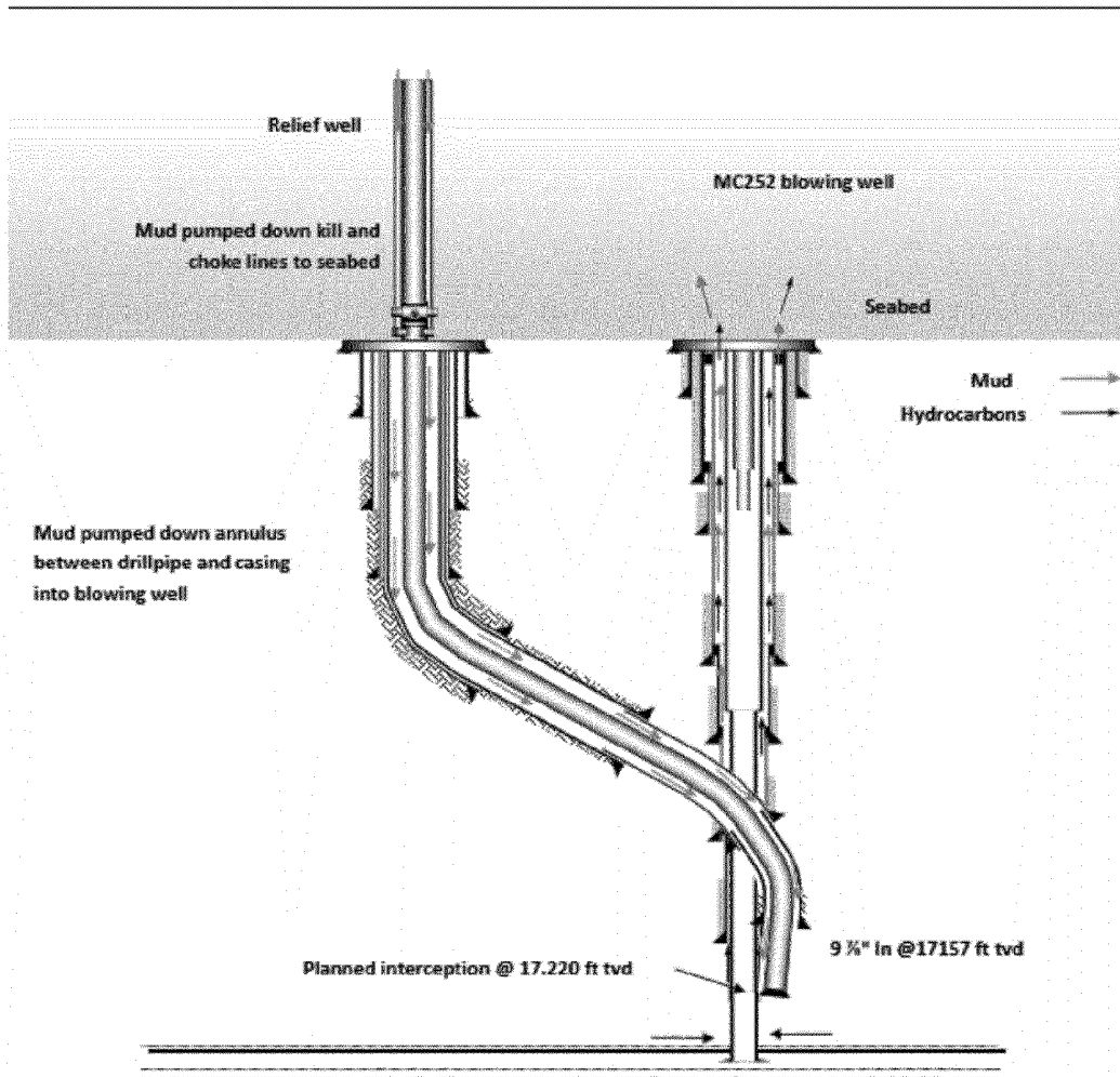
Figure 7: Sketch of relief well pumping operation
