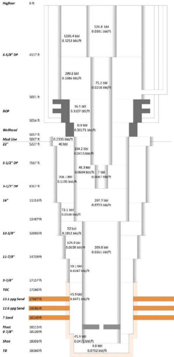
Figure 1.7: Well schematic showing volume capacities
