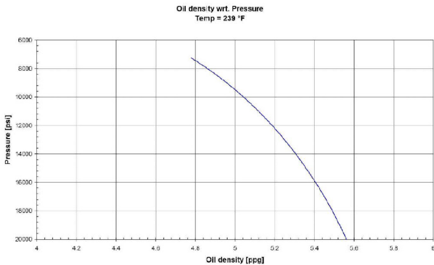
Figure 3.1: Oil density versus pressure for temperature = 239 °F
