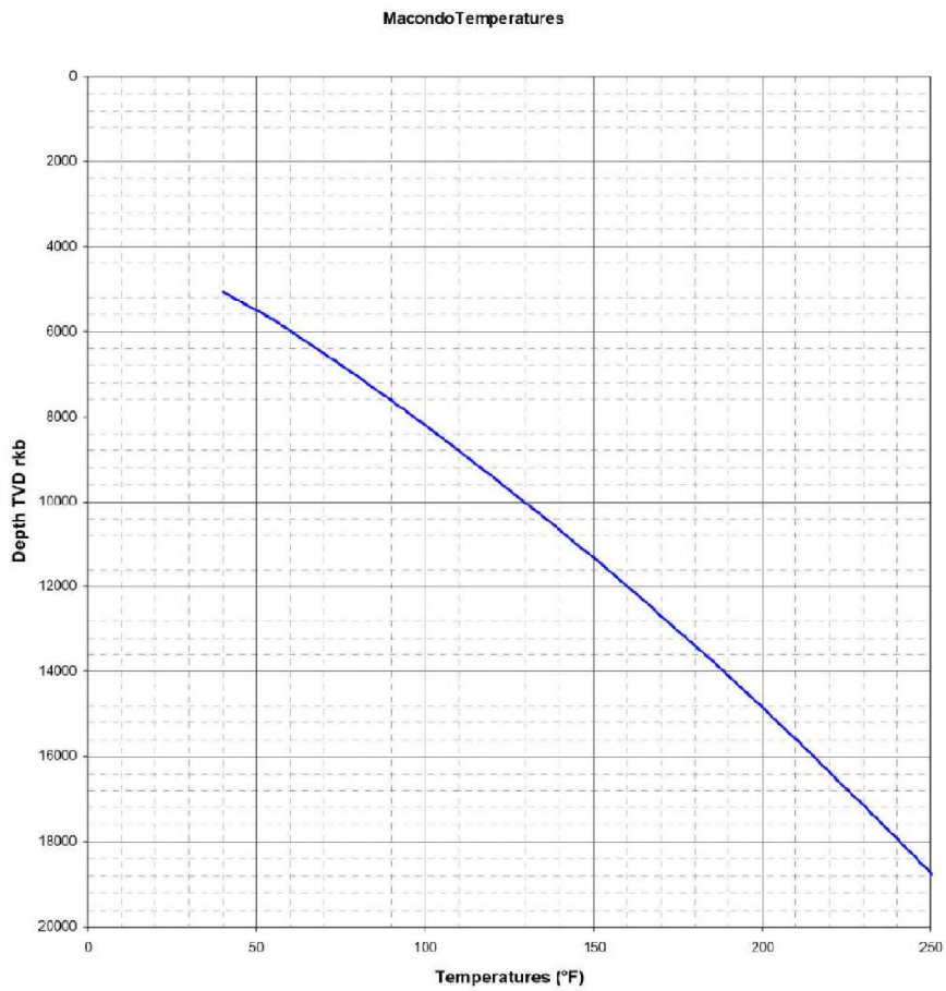
Figure 1.5: Temperature profile
