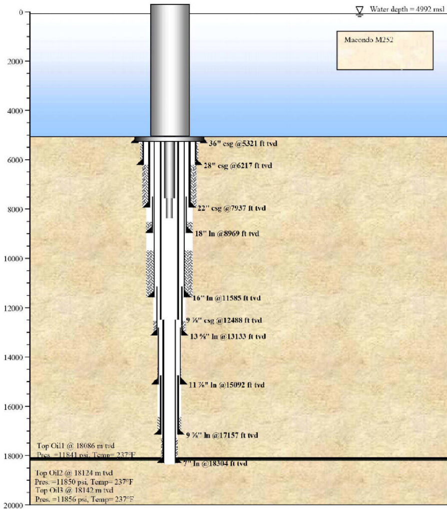
Figure 1.6: Well schematic, TVD drawn to scale
