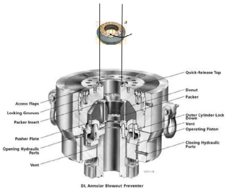
Figure 3.24: Annular blowout preventer
