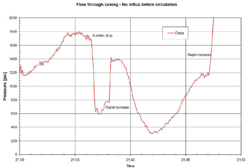
Figure 3.26: Pressure fluctuations the last minutes before explosion
