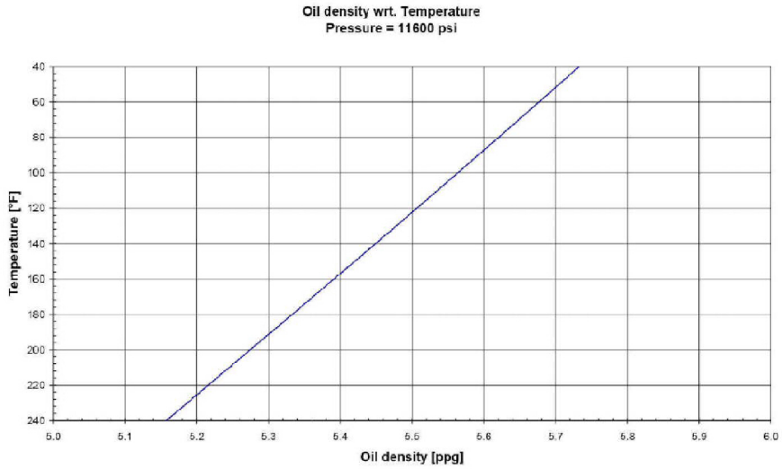
Figure 3.2: Oil density versus temperature for pressure = 11,600 psia
