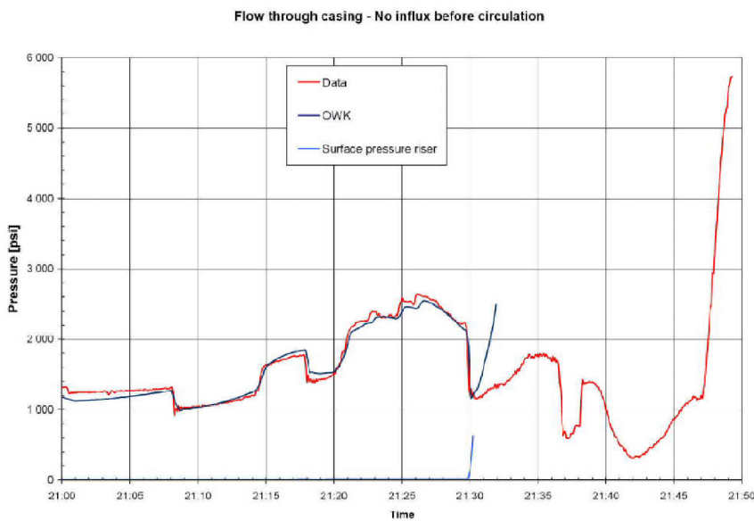
Figure 3.27: Case 5 - Pressure response for a sudden shut-in at surface (no flow)
