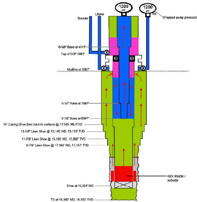
Figure 3.15: Kick and shut-in pressures
