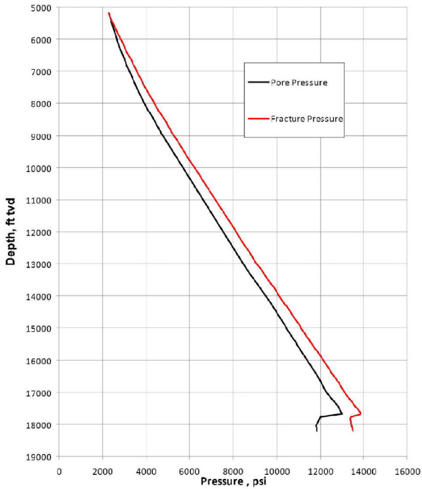
Figure 1.3: Pore and fracture pressure profile
