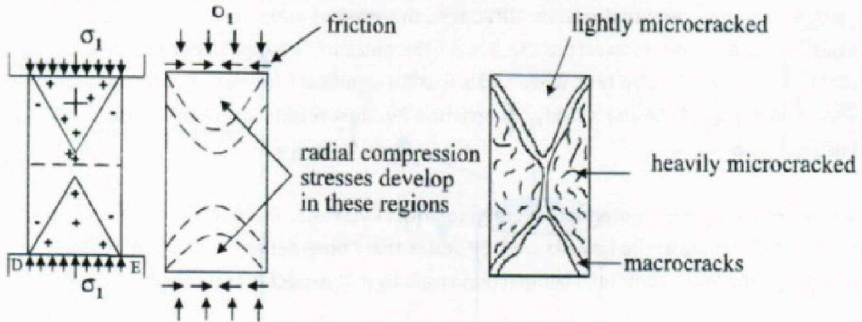
FIGURE 7. Diagram Illustrating End Effects and Friction Cones.
