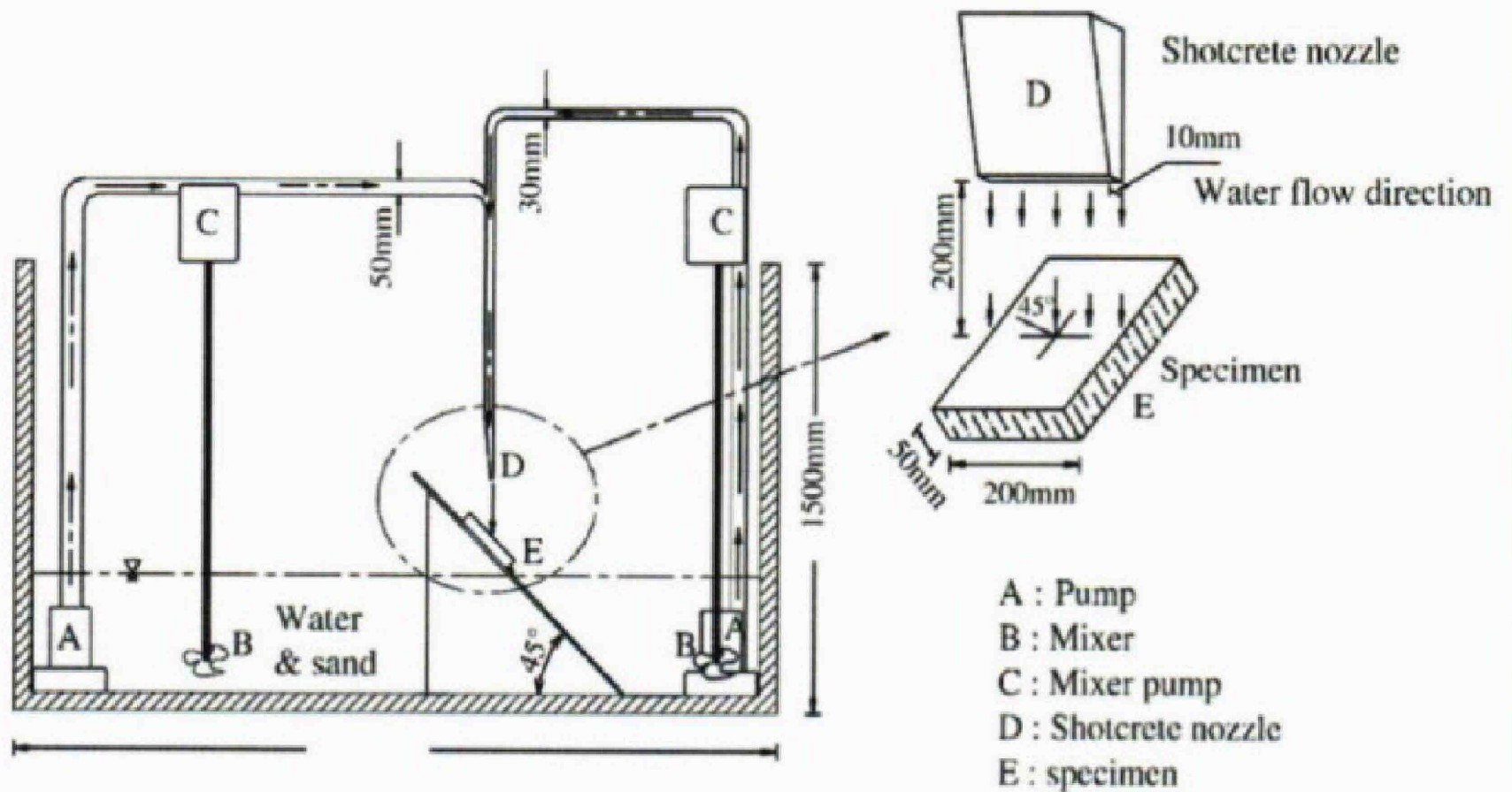
Fig. 3. Water-borne sand abrasion erosion test apparatus.
