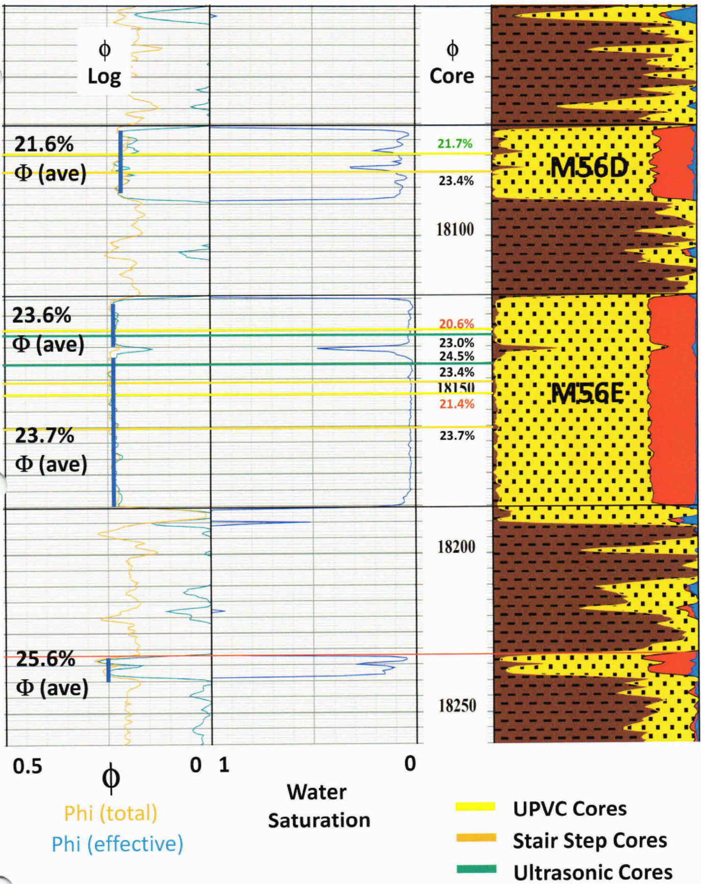
Average Reservoir Porosity From Logs
