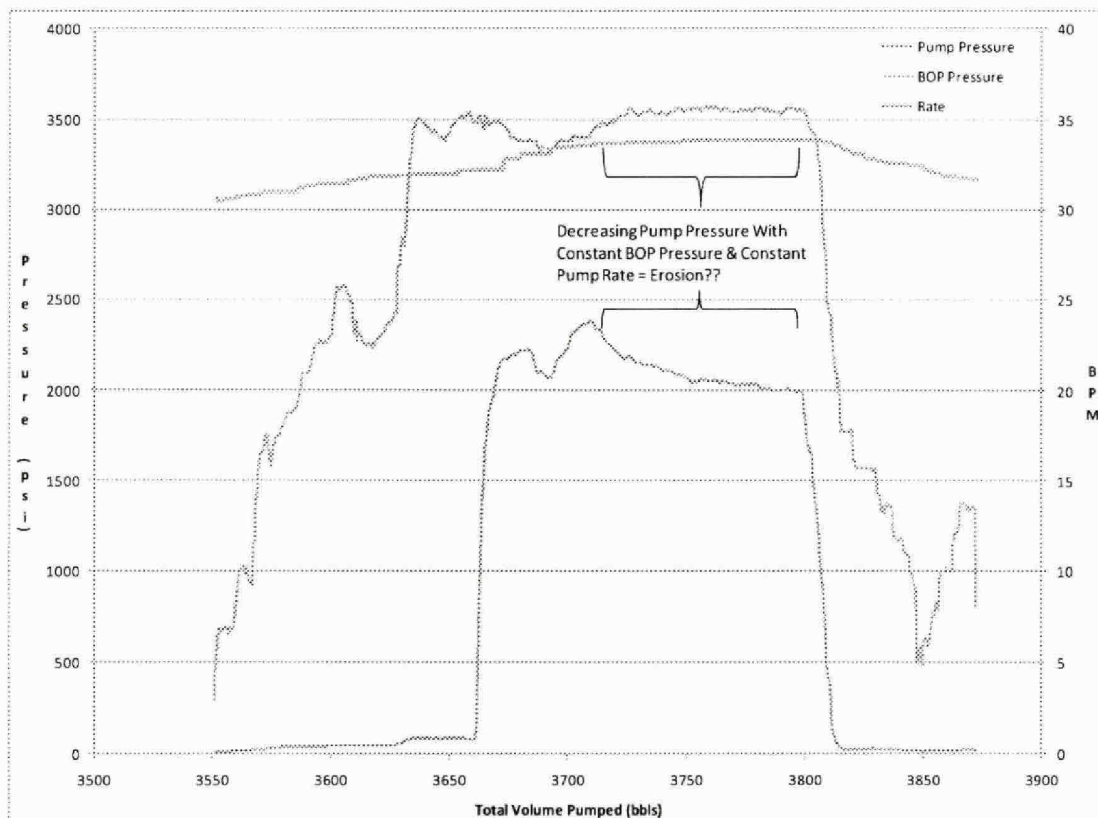
Figure 4.0 - Kill Attempt No. 3 Recorded Data
