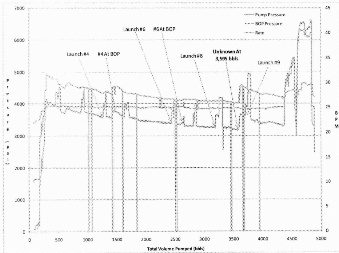
Figure 6.0 - Kill Attempt No. 5 Recorded Data
