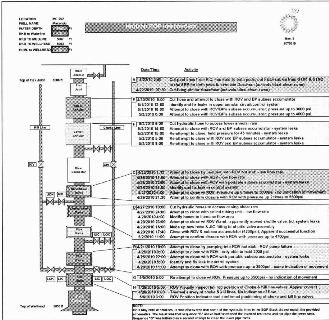
Figure 1.0 – BOP Stack
