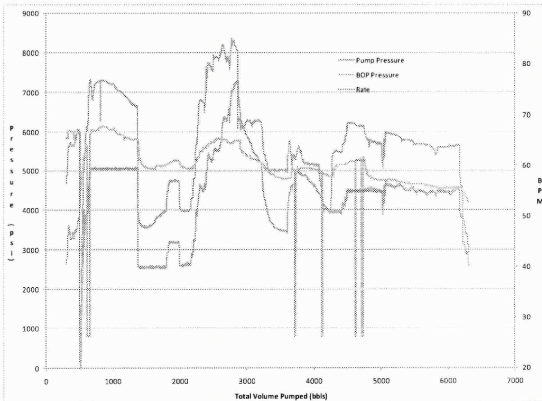
Figure 2.0 – Kill Attempt No. 1 Recorded Data
