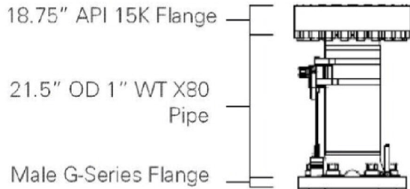
Figure 12 - Transition Spool Components
