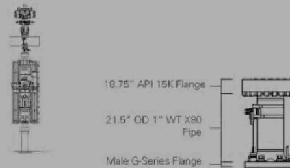
Figure 12 - Transition Spool Components
