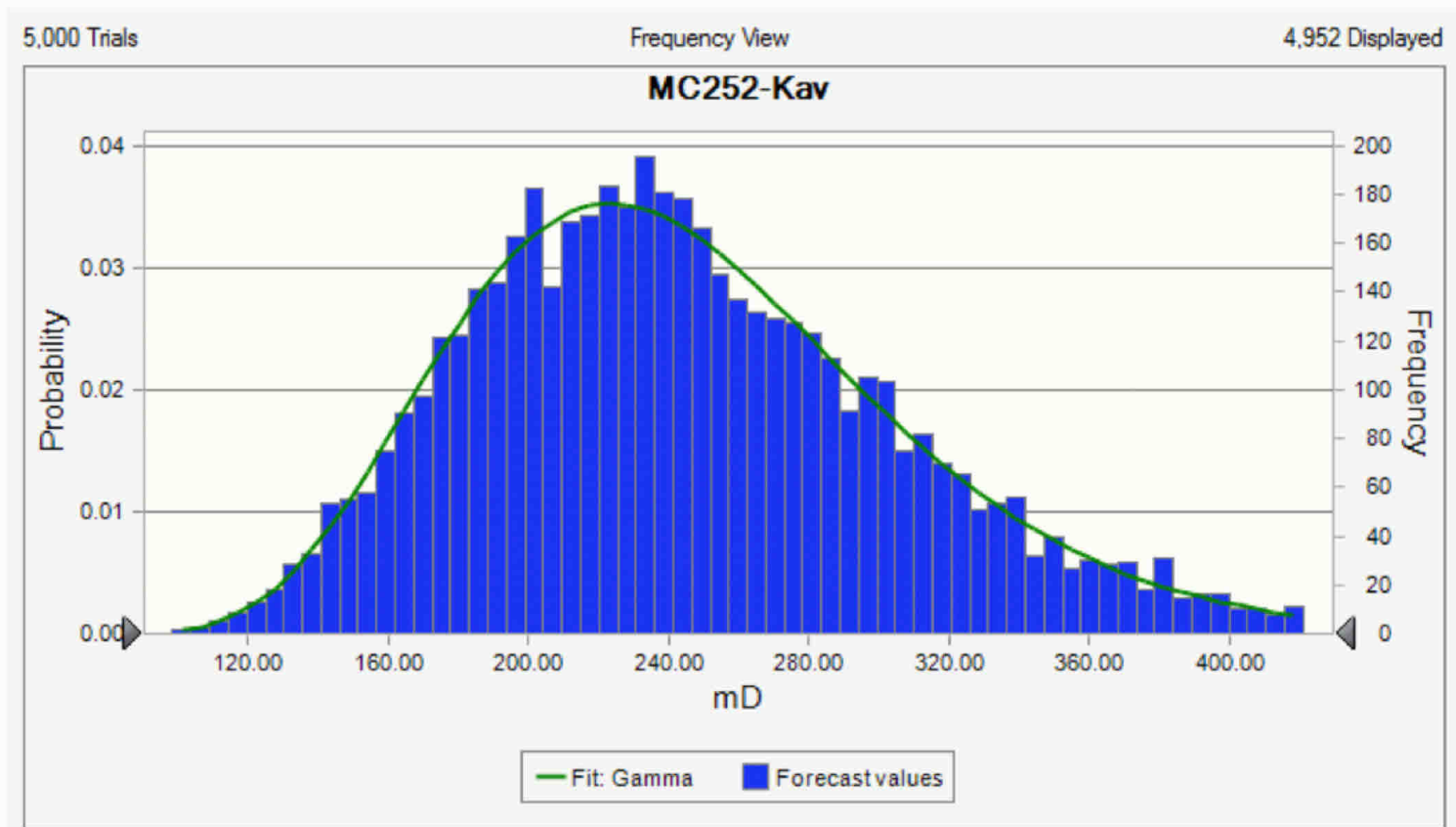
Figure 43: Macondo Permeability – Probability Distribution
