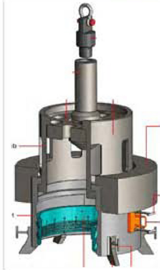
Flange Overshot
