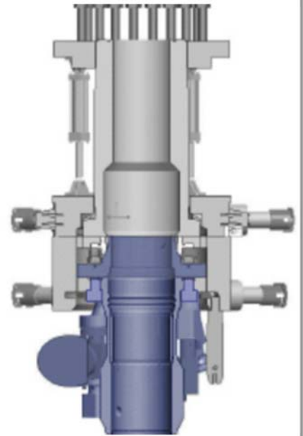
Latch Cap
