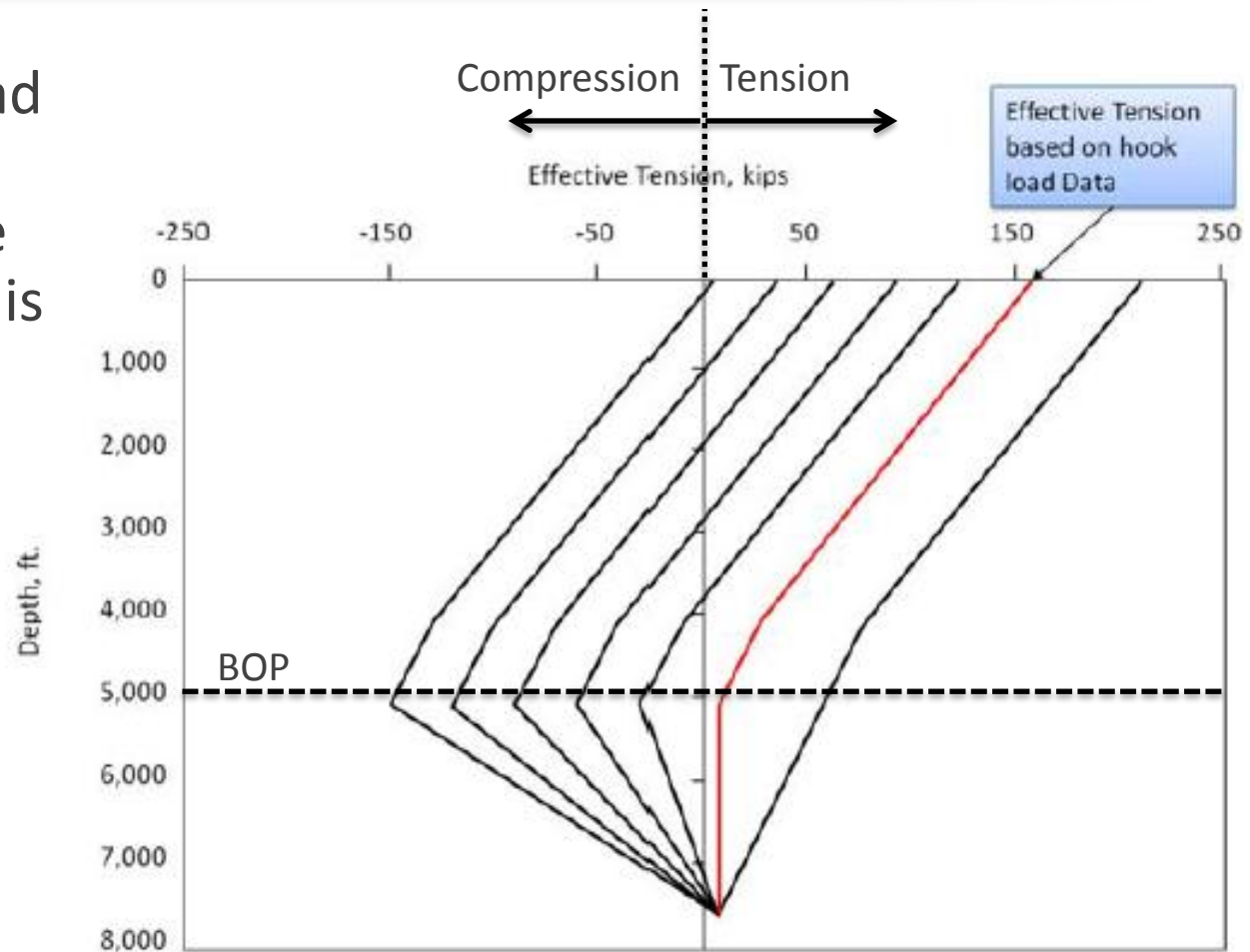
Figure 18 Recreation of Stress Engineering’s Effective Tension Graph
