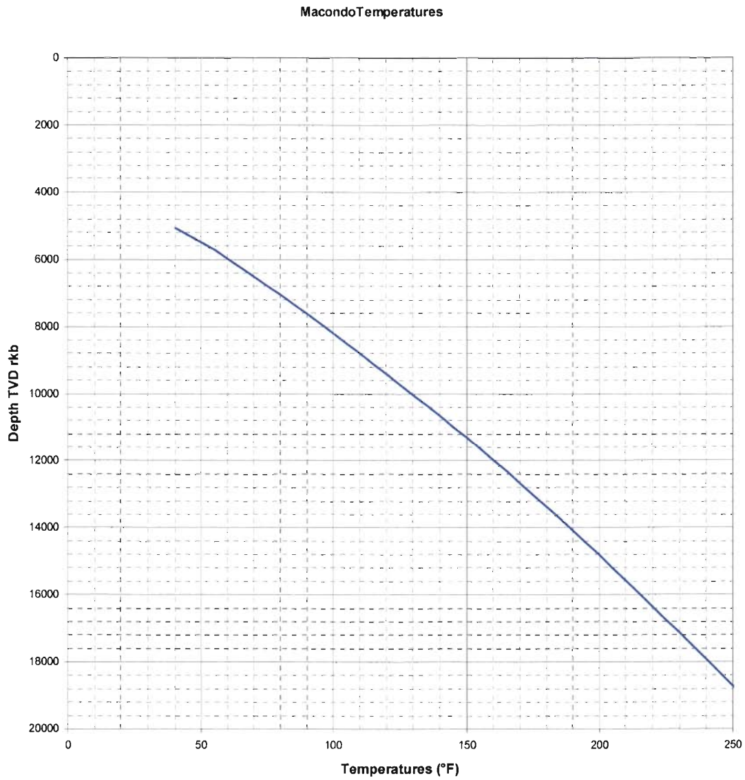
Figure 1.5: Temperature profile
