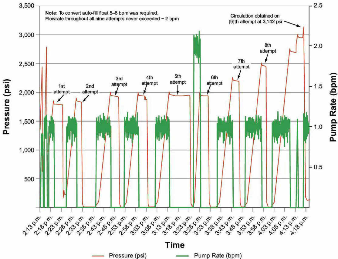
Figure 14: Nine Attempts Prior to Assumed Conversion of Float Collar on April 19, 2010 (Figure 13 from Transocean Report, Alteration Added) 104
