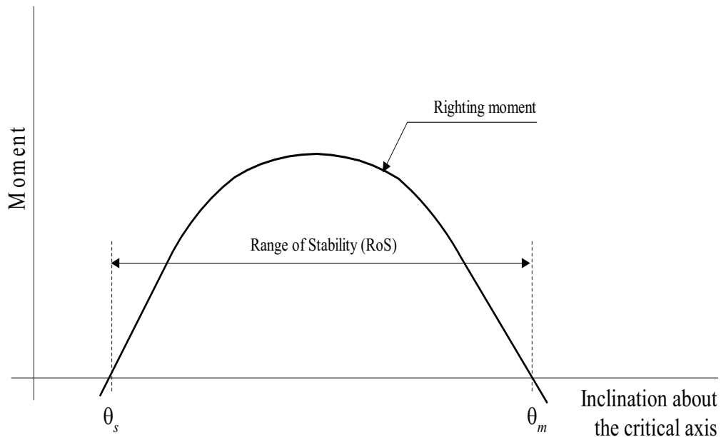
Figure 3-2 – Residual stability for self-elevating units
