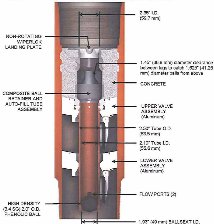
Figure 11: Weatherford M45AP Float Collar Used In Macondo Well 97
