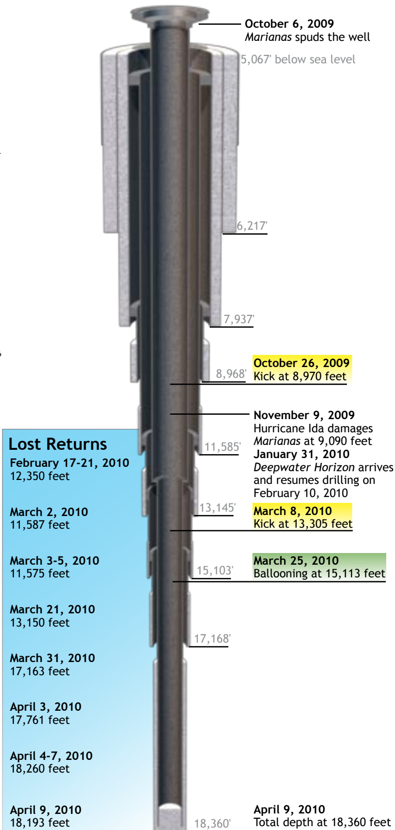
Figure 4.2.8. Timeline of drilling events.
