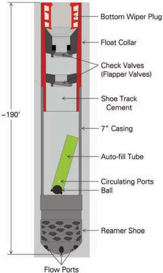
Figure 4. Shoe Track.
