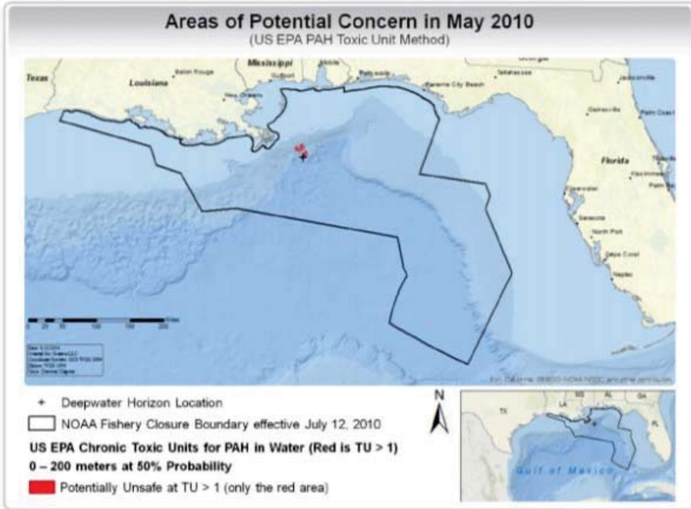
Figure 14. This map shows the maximum NOAA fishery closure area (boundary drawn with black line) compared to the most conservative estimate of the area that is potentially harmful to aquatic life. See Appendix I for a description of the methodology used to map the area of potential harm.
