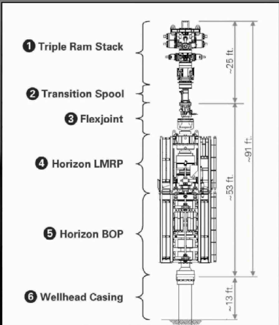
Figure 1 - Components
