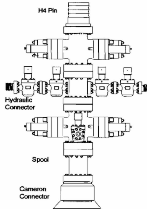
Capping BOP
