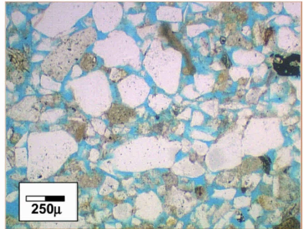
Higher quartz rock, approaching Macondo percentage of 93%
