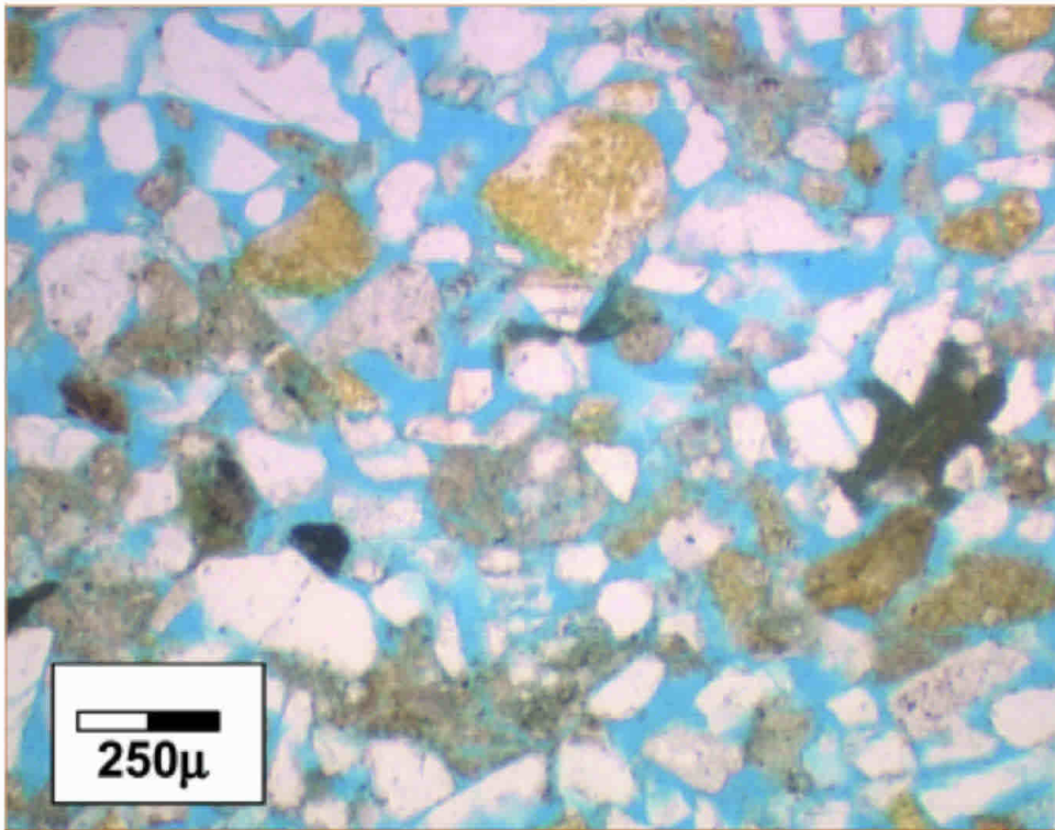
Non-Macondo type rock: Higher percentage dark “ductile” minerals
