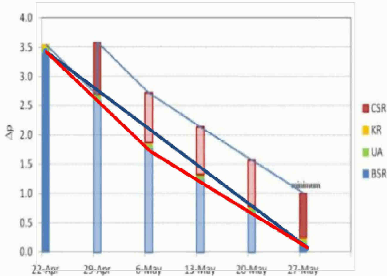
Figure 33. Normalized change in pressure drop seen for individual components and the cumulative change in the overall pressure drop, April 22- May 27, 2010.
