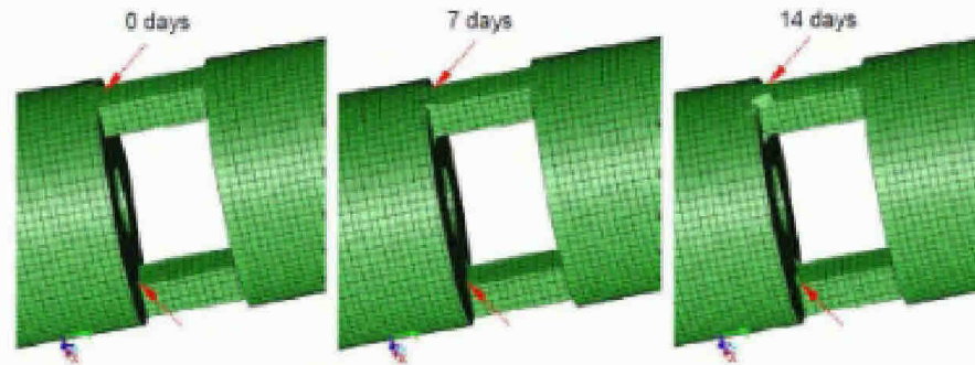
Figure 30. Transient simulation showing erosion of BSR flow geometry; red arrow points to locations of maximum erosion.
