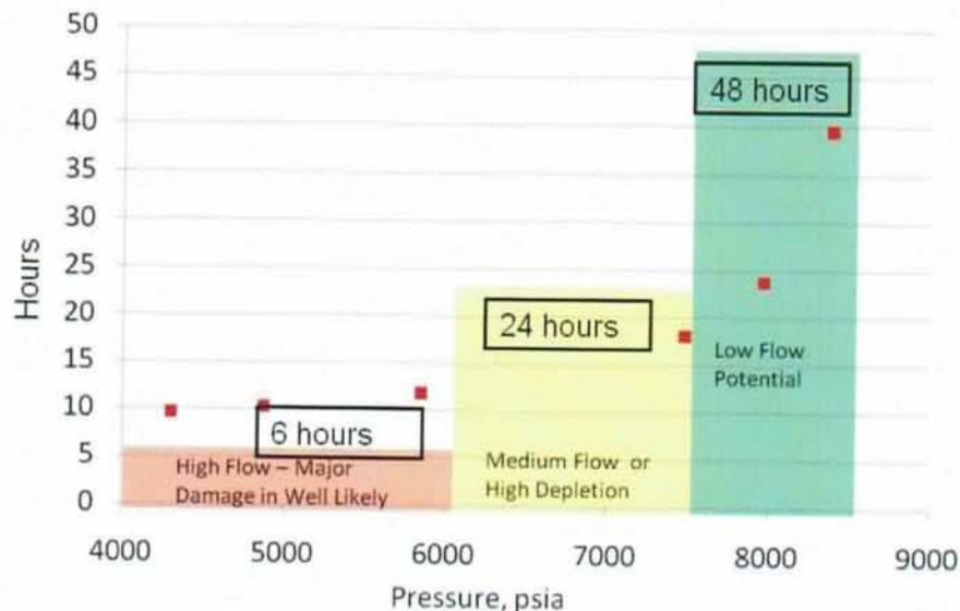
Figure 2: Well Integrity Test Duration Guidance
