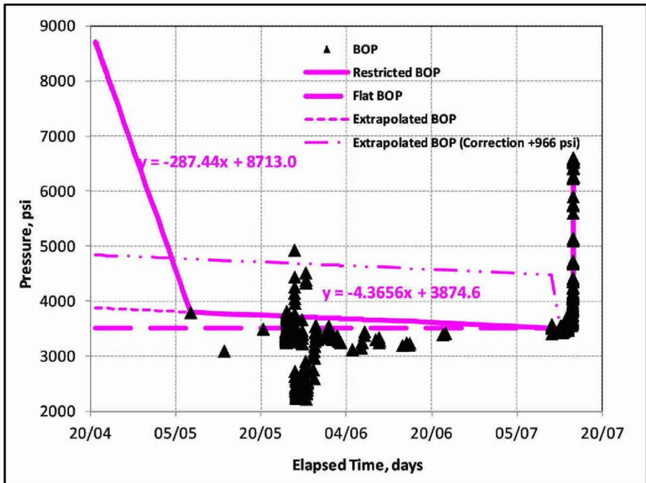
Figure 16: Recorded BOP pressure between May 8 and July 15, indicating erratic and sparse values prior to the integrity test. Also shown are the four sensitivity cases
