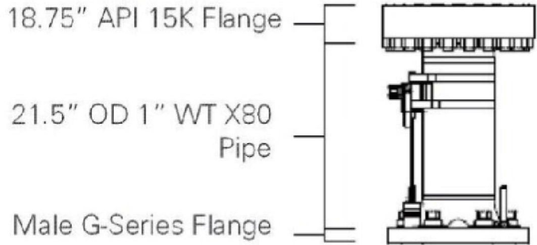
Figure 12 - Transition Spool Components
