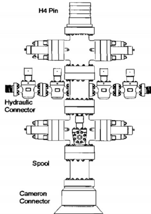
Capping BOP
