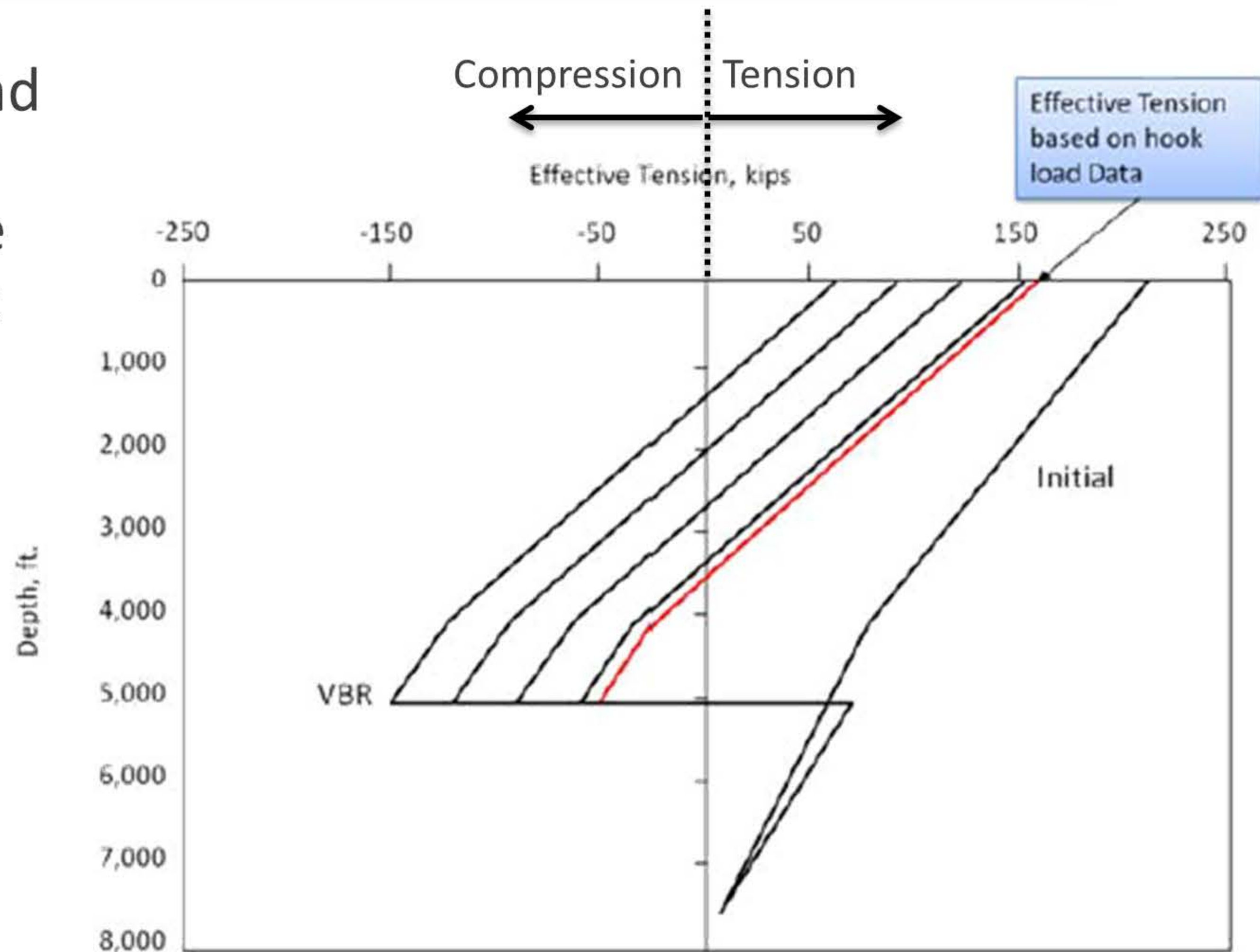
Figure 19 Recreation of Stress Engineering’s Effective Tension Graph
