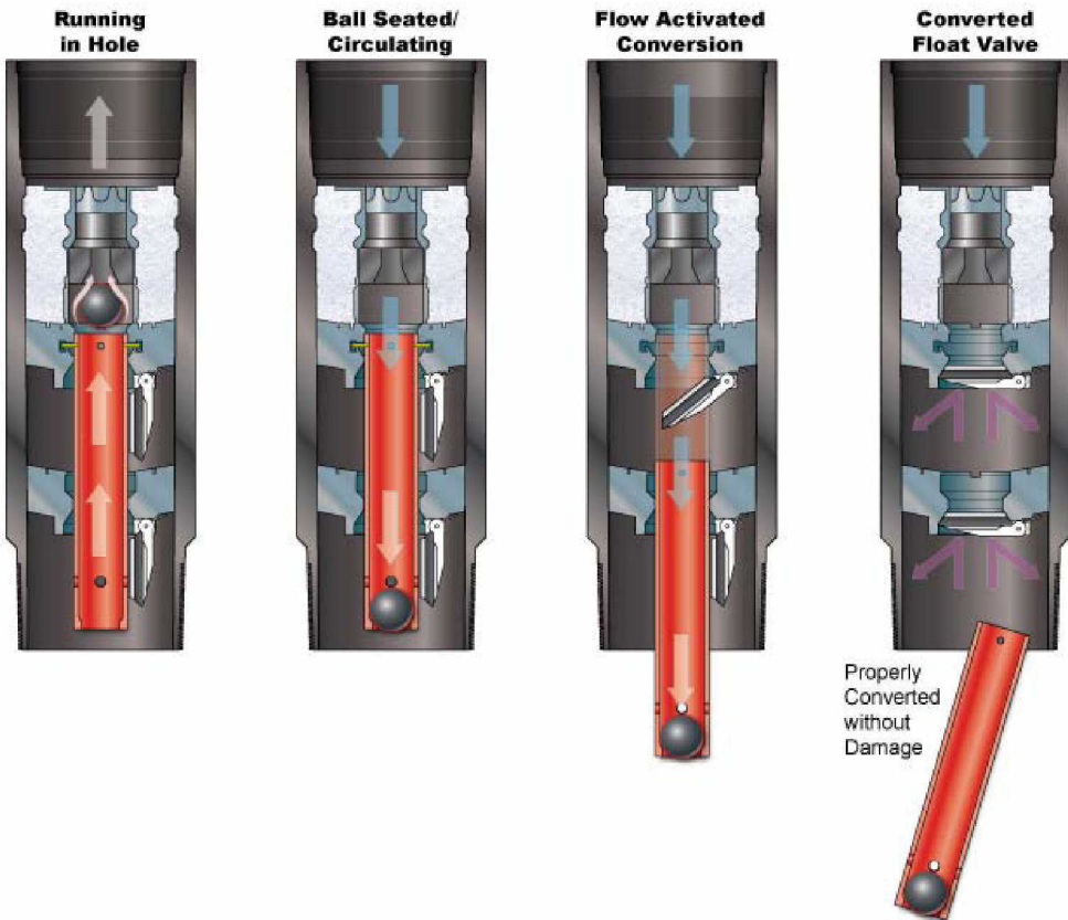
Figure 12: Flow-Activated Auto-Fill Float Collar Properly Converted Without Damage
