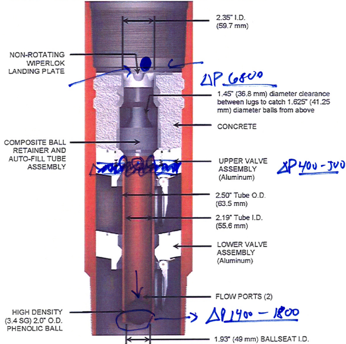
Figure 11: Weatherford M45AP Float Collar Used In Macondo Well 97
