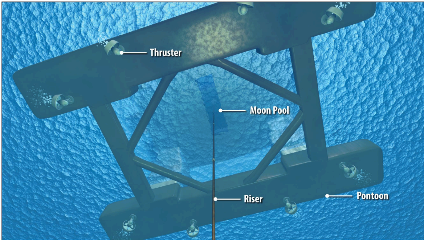
Figure 3.5. Subsurface portion of the Deepwater Horizon .
