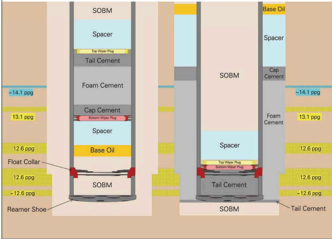
Figure 3. Planned Cement Fluid Locations.
